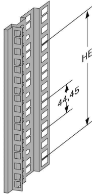
19" Rasterholme
