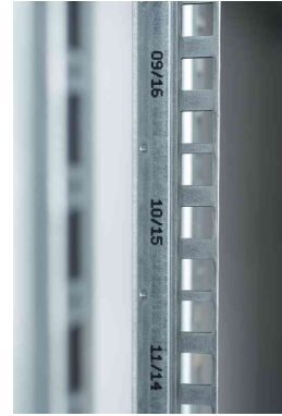
19" Rasterholme
